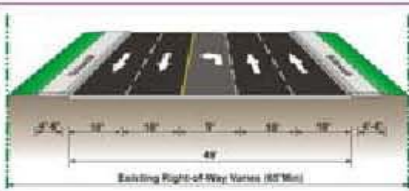
Frierson Ave. to Hillsborough Ave. EXISTING TYPICAL - NO CHANGE
