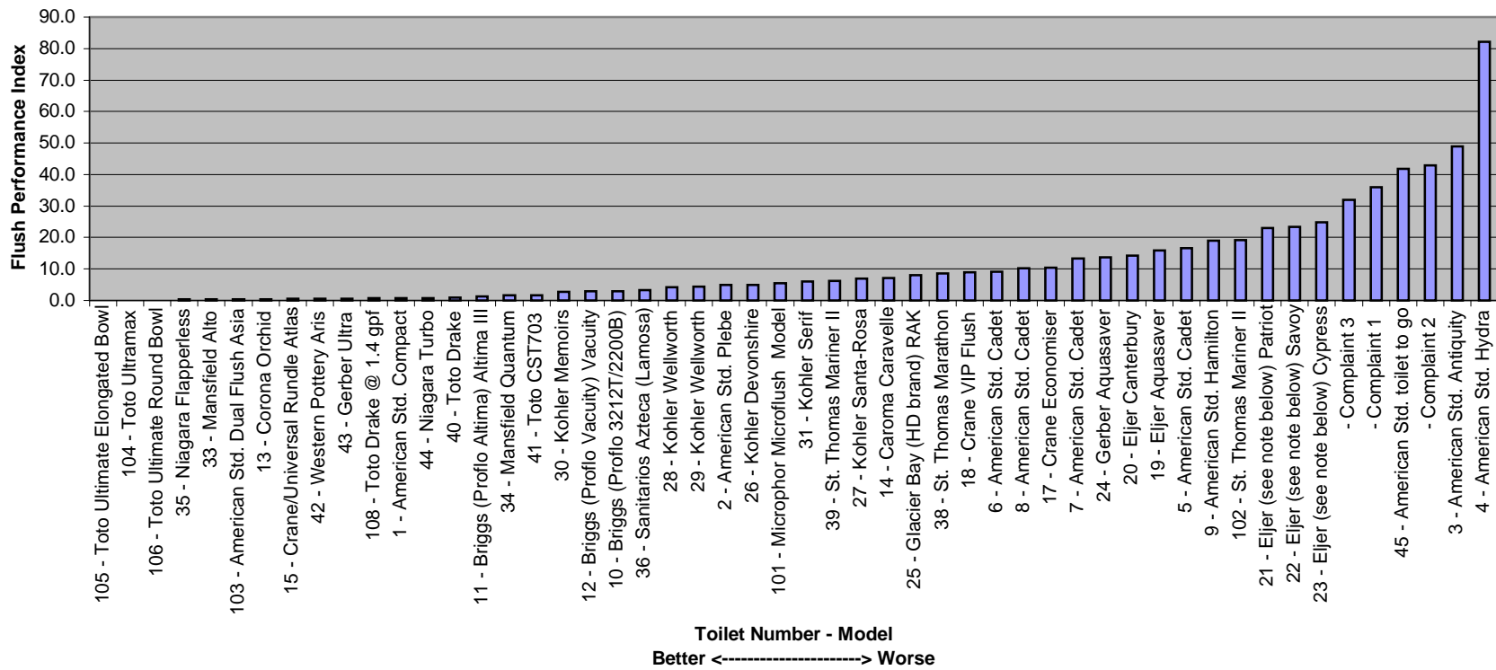
FIGURE 1 FLUSH PERFORMANCE INDEX
