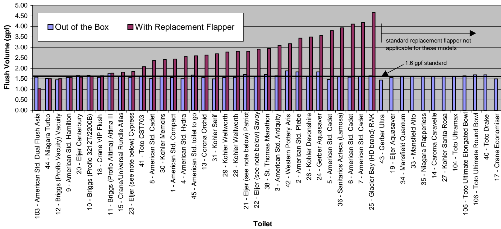
Figure 2 FLUSH VOLUME DISTRIBUTION (1.6 gpf units)
