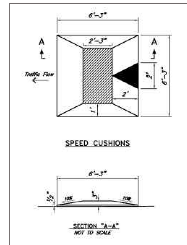
Speed Cushion Details
