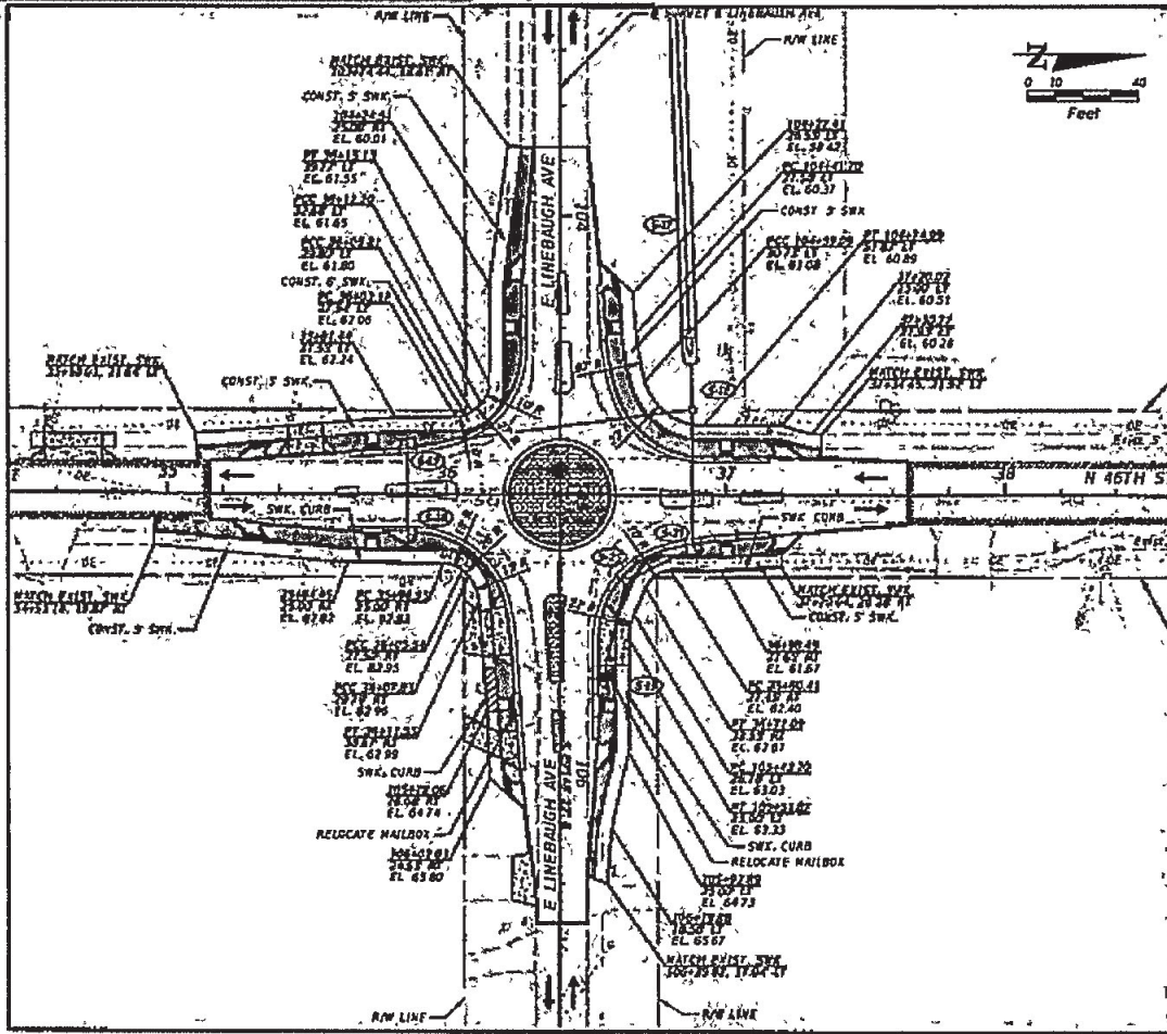
Figure 2- Graphic of proposed mini-roundabout at 46th Street and Linebaugh Avenue.
