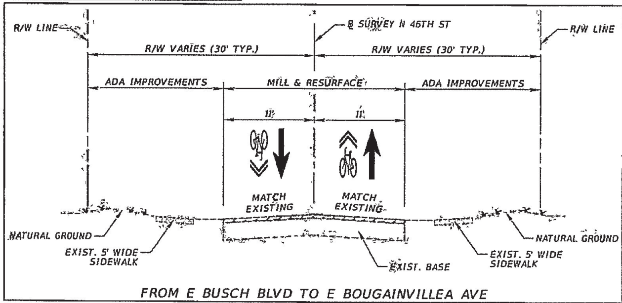
Figure 1- Proposed Typical Cross Section
