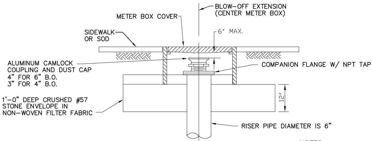
BLOW-OFF OUTLET DETAIL
