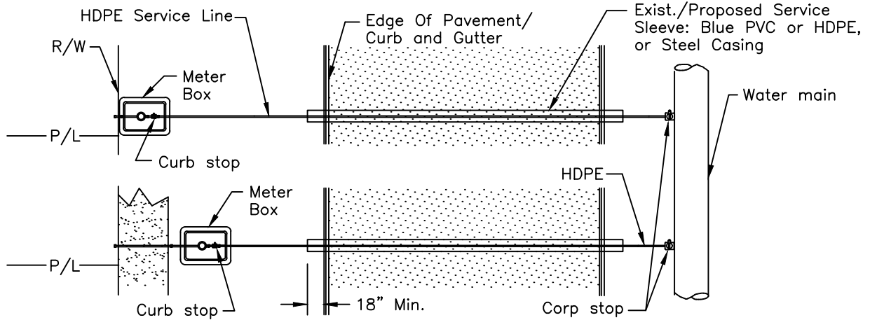
PLAN VIEW - SINGLE METER
