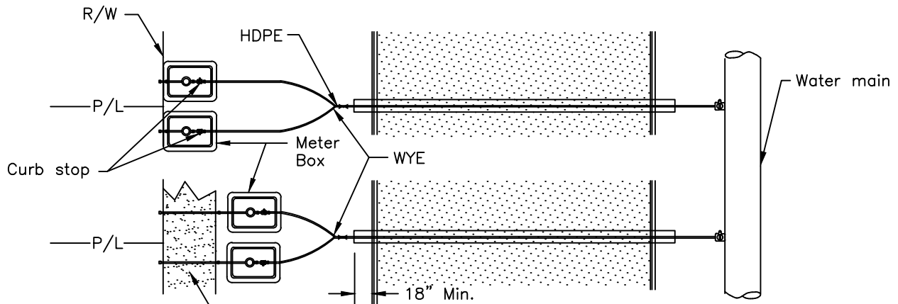
PLAN VIEW - DUAL METER
