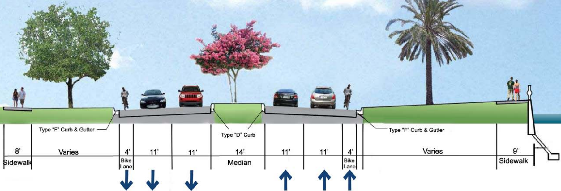
Typical Section 2: Davis Island Bridge to Rome Avenue
